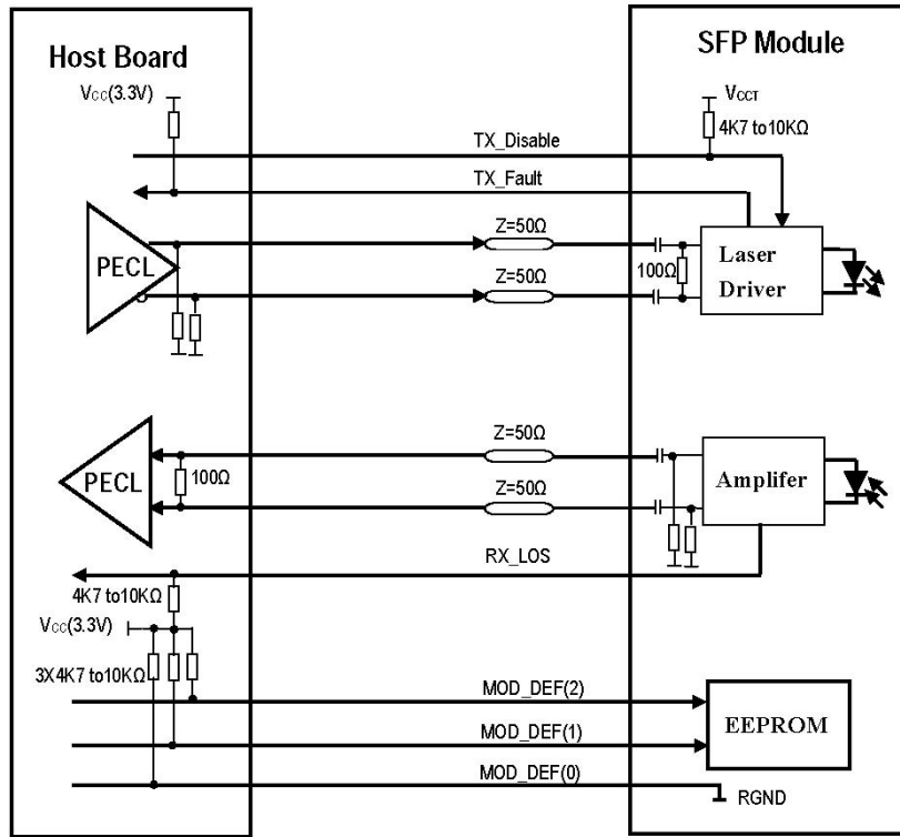
Recommended High-speed Interface Circuit
