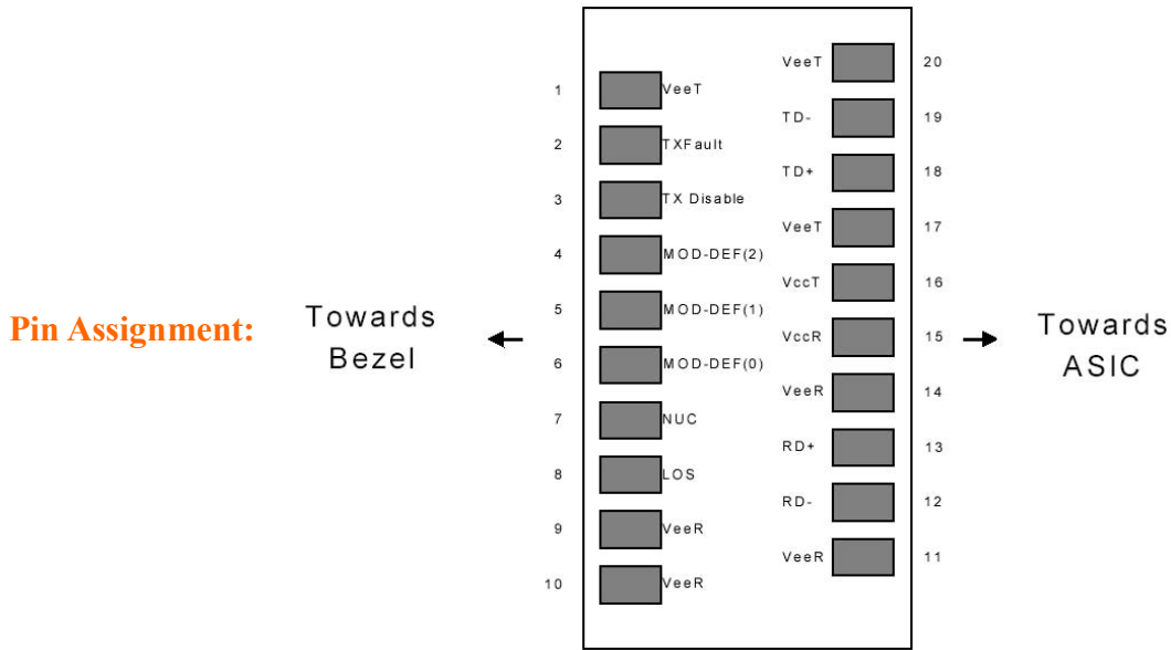
Diagram of Host Board Connector Block Pin Numbers and Names
