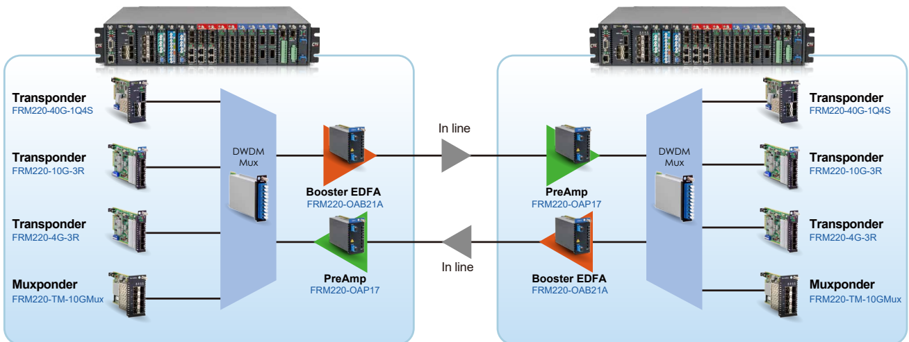
CWDM /DWDM P to P Application
