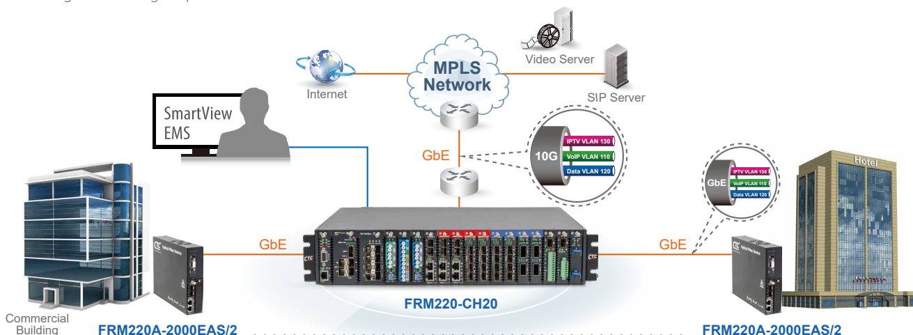
Typical FTTB Application
