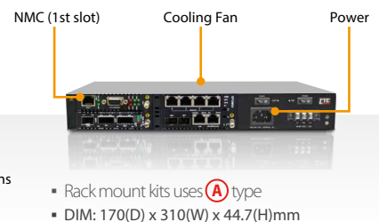
CH04A (1U 4 Slots)
