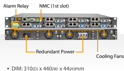
CH08 (1U 19" 8 Slots)
