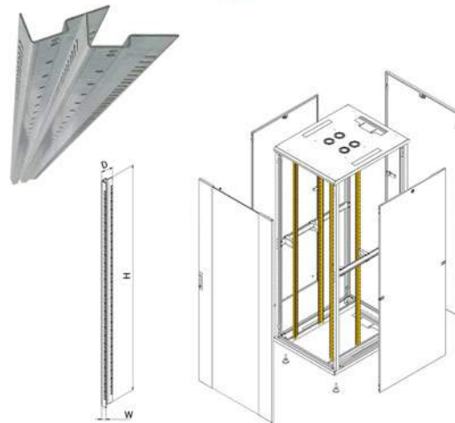
Component Position
