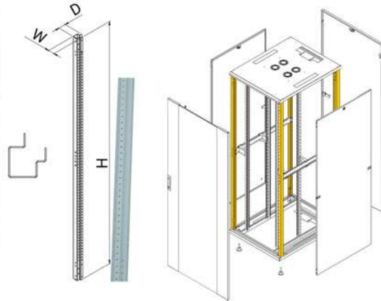
Component Position
