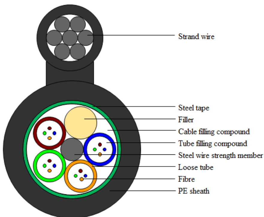
GYTC8S-16B1.3
